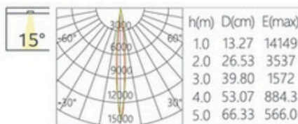
Narrow Spot 15°
