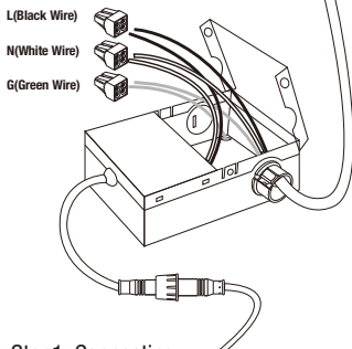
Step1: Connecting
