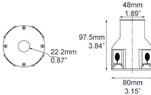
MOUNTING SLEEVE
