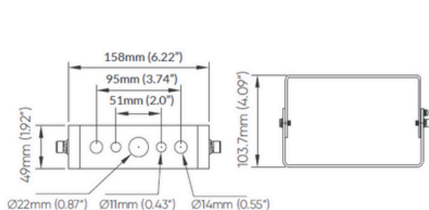
Yoke (100W/150W/200W/300W)
