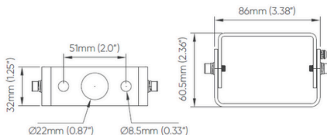
Yoke (30W/60W)
