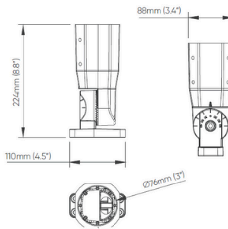
Ø70mm Slipfitter (100W/150W/200W/300W)
