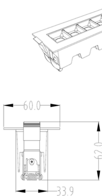
5 Cells Linear Downlight White Body
