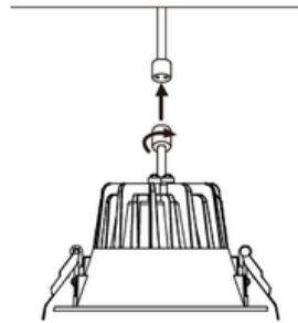
Step3: Twisting
