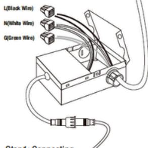
Step1: Connecting
