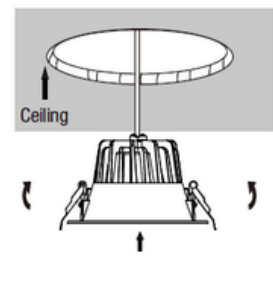
Step4: Pushing
