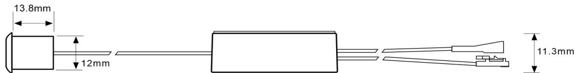
SIDE VIEW
