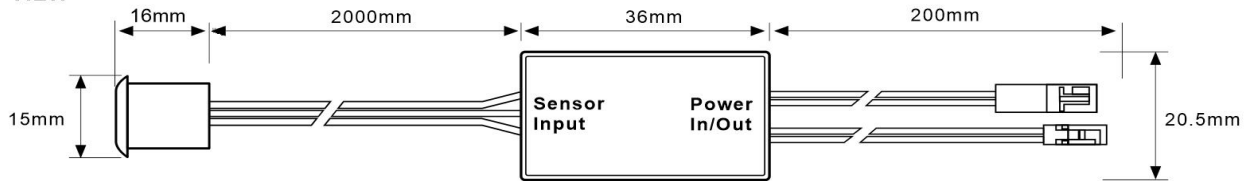
TOP VIEW
