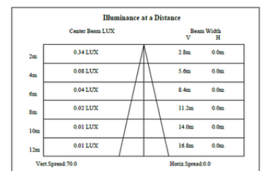
Lux distance Curve
