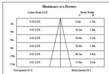
Lux distance Curve
